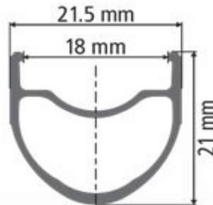
RR411 rim dimensions- rim brake
