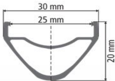
XM421 rim dimensions
