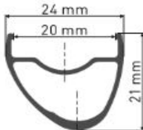
RR421 rim dimensions- disc asym
